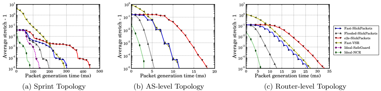
Figure 8: Average packet stretch - 1 vs. packet generation time when t_0 = 0 . The y-axes are on log scales. For the Sprint topology, D = 50, d_r = 2 . For the AS- and router-level topologies, D = d_r = 0 .
