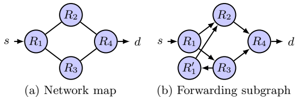
Figure 2: An FS may have multiple representations of a network map node, to allow “backtracking” without introducing cycles in the FS.
